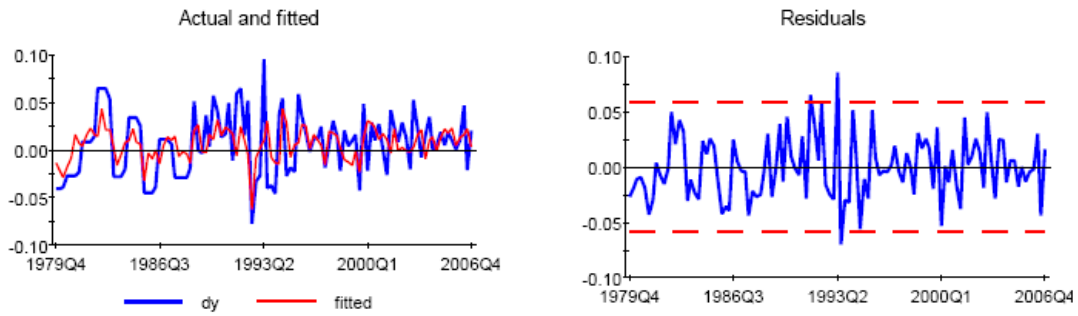
Figure 12: Actual, Fitted, and Residuals for the Core Equations
