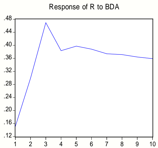
ALGERIA: impulse response function
